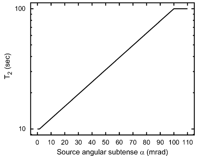
Fig. 5. The time T_2 indicates the transition between the exposure duration dependent exposure limit for extended sources and exposure duration independent exposure limit for constant irradiance for exposure durations greater than T_2 .
